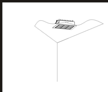
The lamp and drive into the frame, hear "click" sound, see the lamp is stable;
