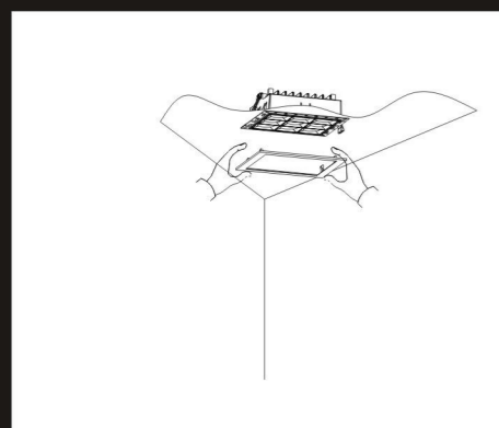
Connect the lamp driver to the end of the line;
